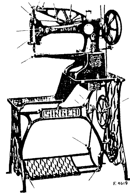
FIG. 10. OILING PLACES IN MACHINE AND STAND
