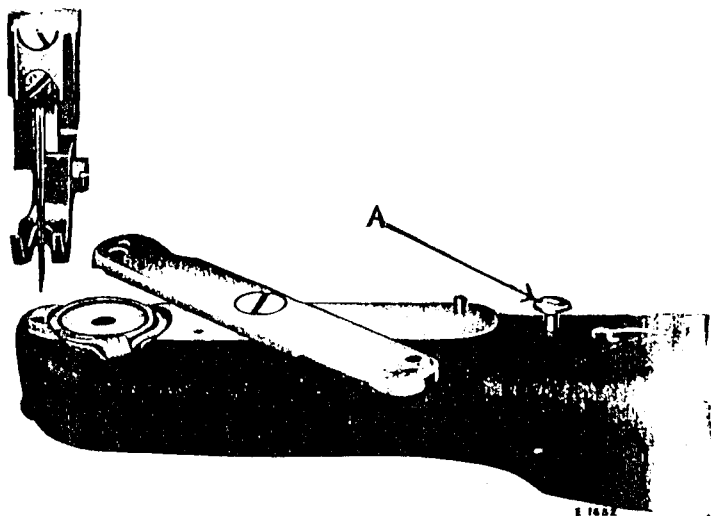
FIG. 3. TAKING OUT THE SHUTTLE
