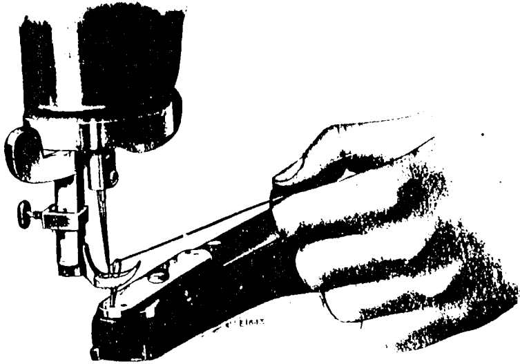
FIG. 12. DRAWING UP OF THE UNDER THREAD
